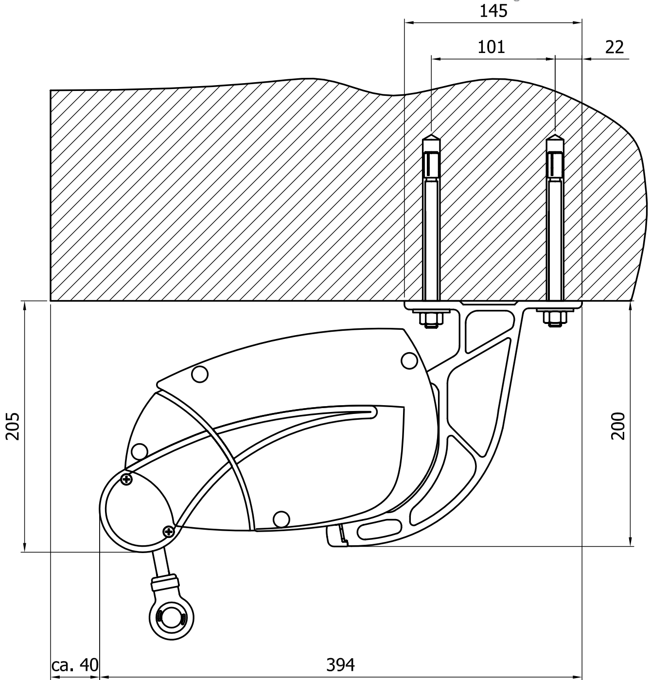
HELIOSHADE CASSETTE - TOP FIX (SHOWN WITH OPTIONAL FRONT VARIO VALANCE)
