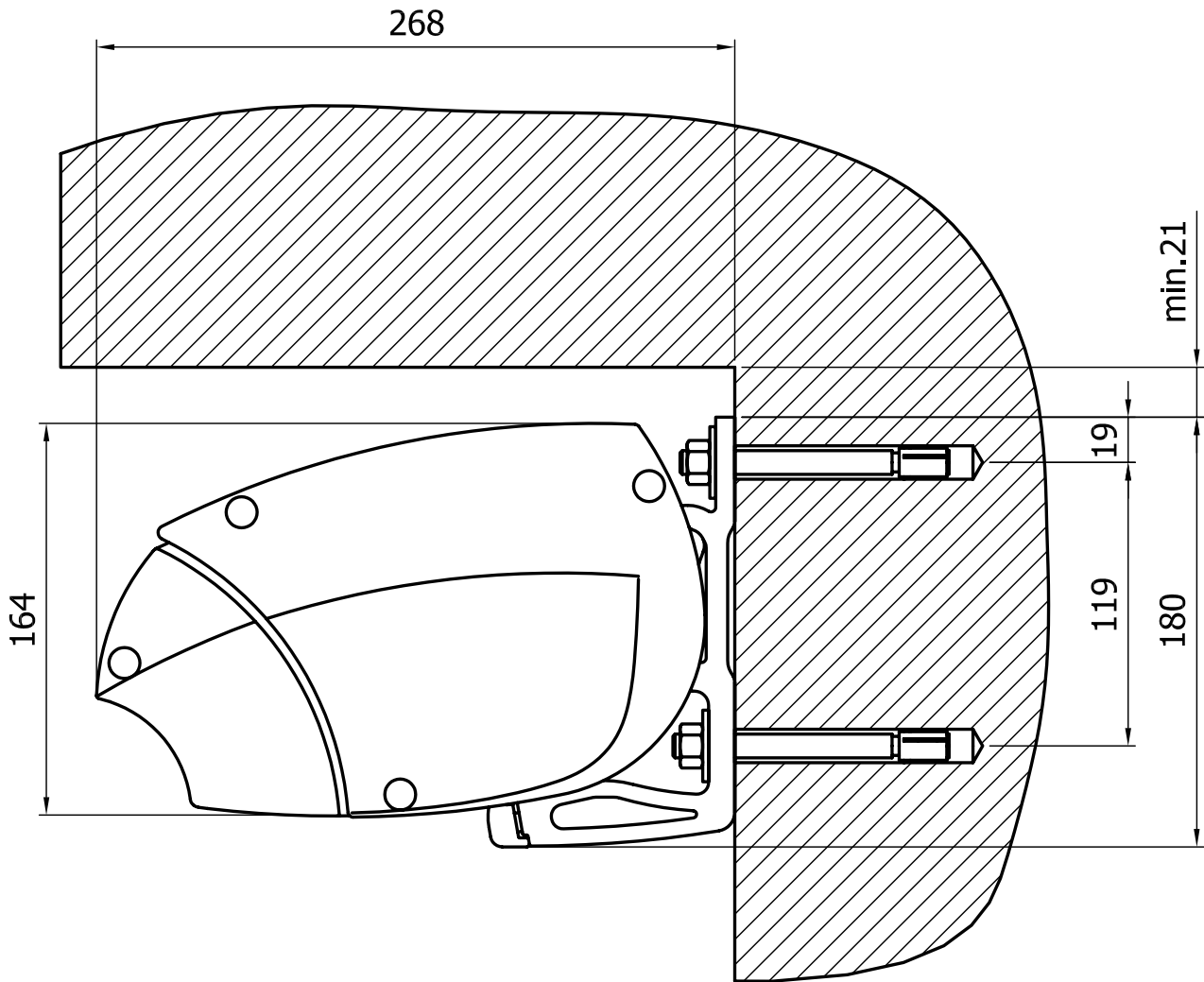
HELIO SHADE CASSETTE - FACE FIX
