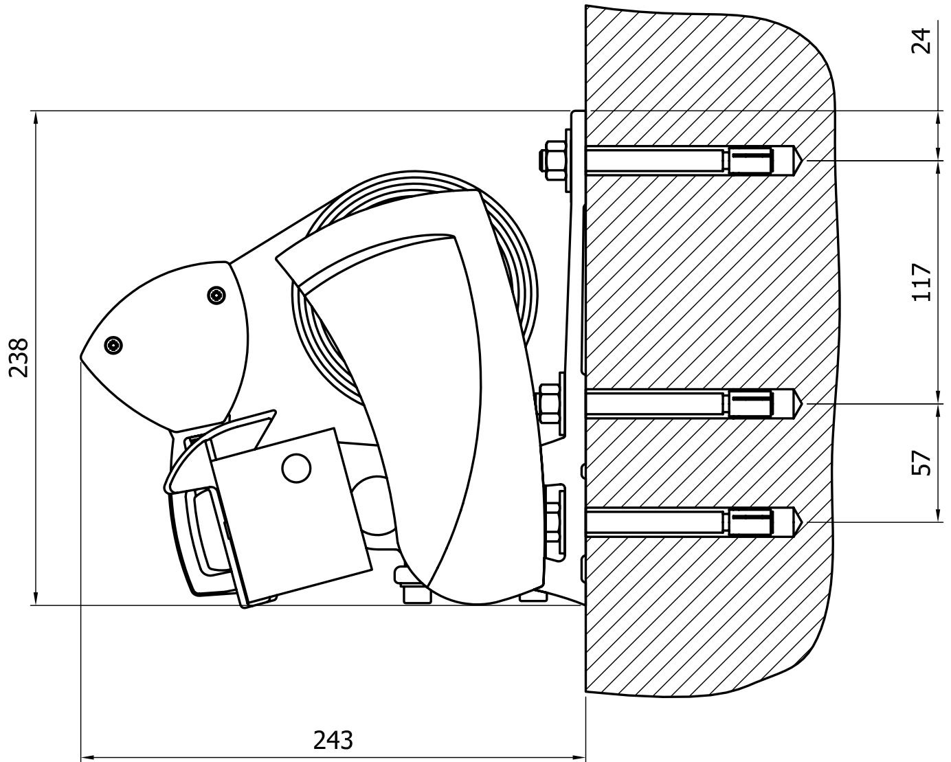
HELIO SHADE CLASSIC - FACE FIX (WITH OUT PELMET)
