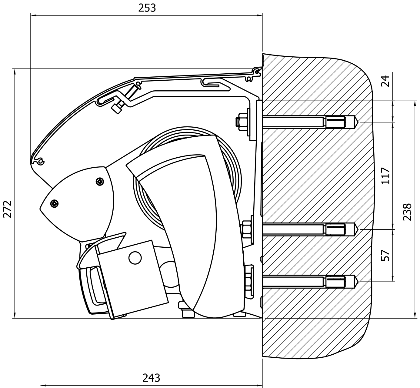
HELIOSHADE CLASSIC - FACE FIX (WITH PELMET)
