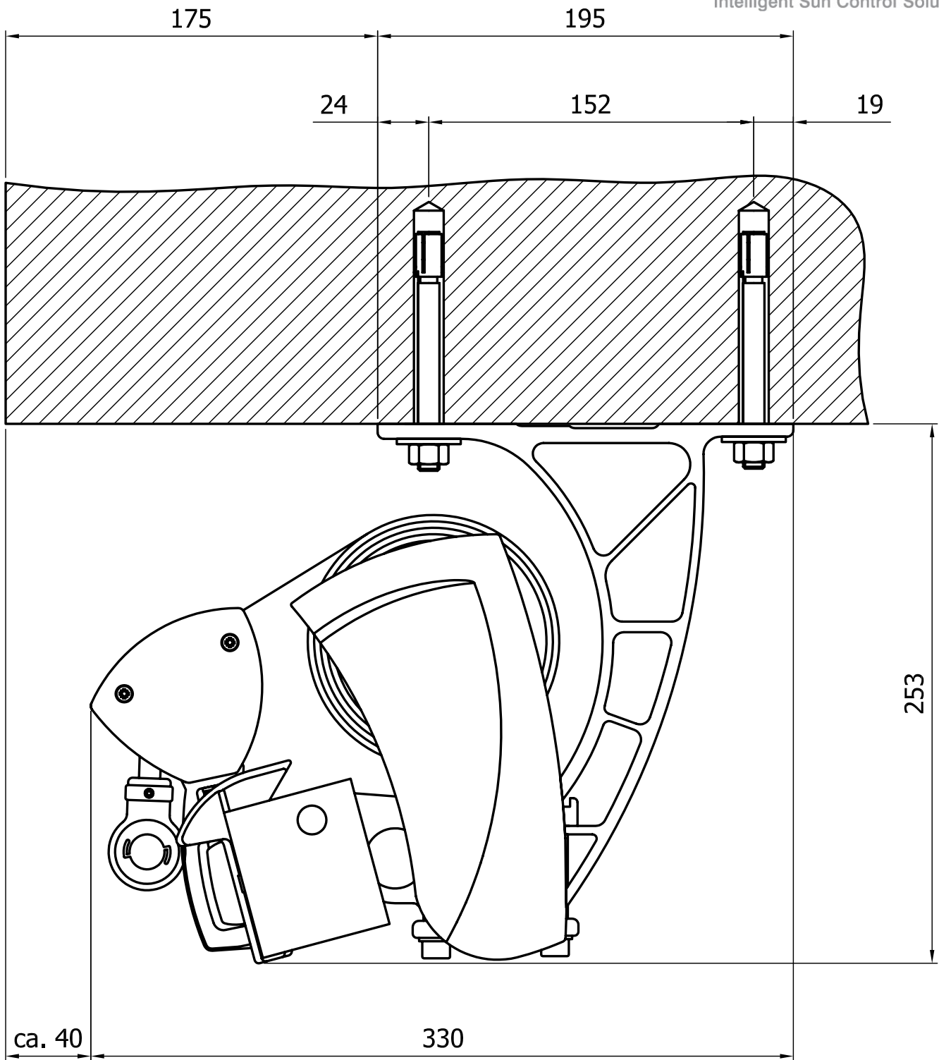
HELIO SHADE CLASSIC - TOP FIX
